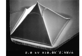
SEM micrograph of the sharpened pyramidal tip
